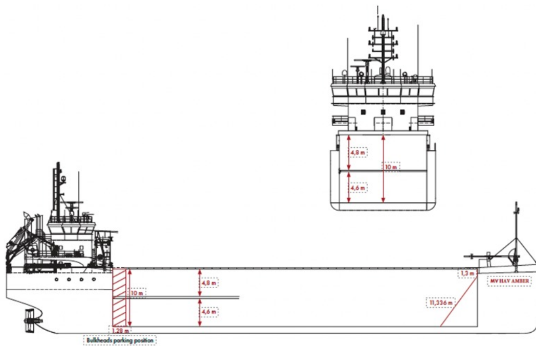
Main Deck
